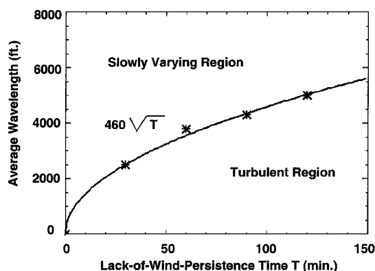
Fig. 3 Average wavelength boundary between relatively slowly varying components of wind profiles and more rapidly varying, turbulent components. 21
