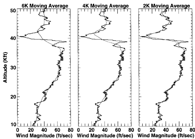
Fig. 1 Effect of different levels of wind smoothing.
