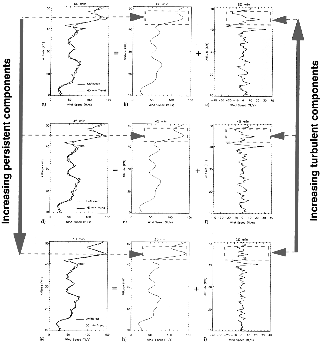
Fig. 2 Typical wind profile. Plots a, d, and g show the average persistent components, for 60-, 45-, and 30-min time periods, superimposed on the measured profile. Plots b, e, and h show the slowly varying components; c, f, and i show the corresponding turbulent components.
